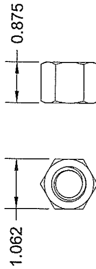
3/4"-10 THREAD W/ NYLON INSERT
