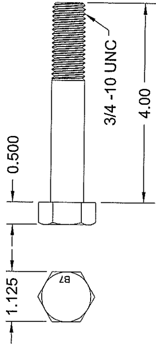
1708-1010-003 HEX BOLT, 3/4 -10 UNC X 4 LG STEEL SA-193, GRADE B7
